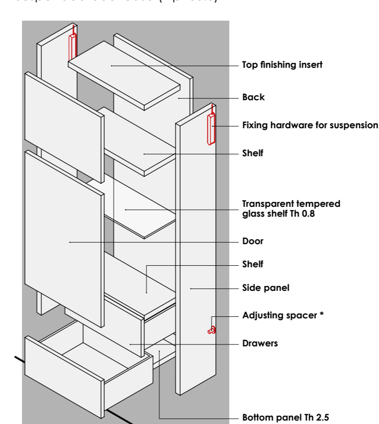
Suspended bookcase (Dpt 33.3)
