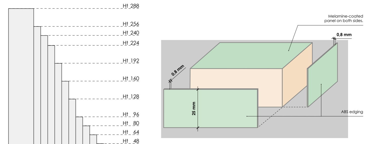
Doors W 45, 50 and 60
