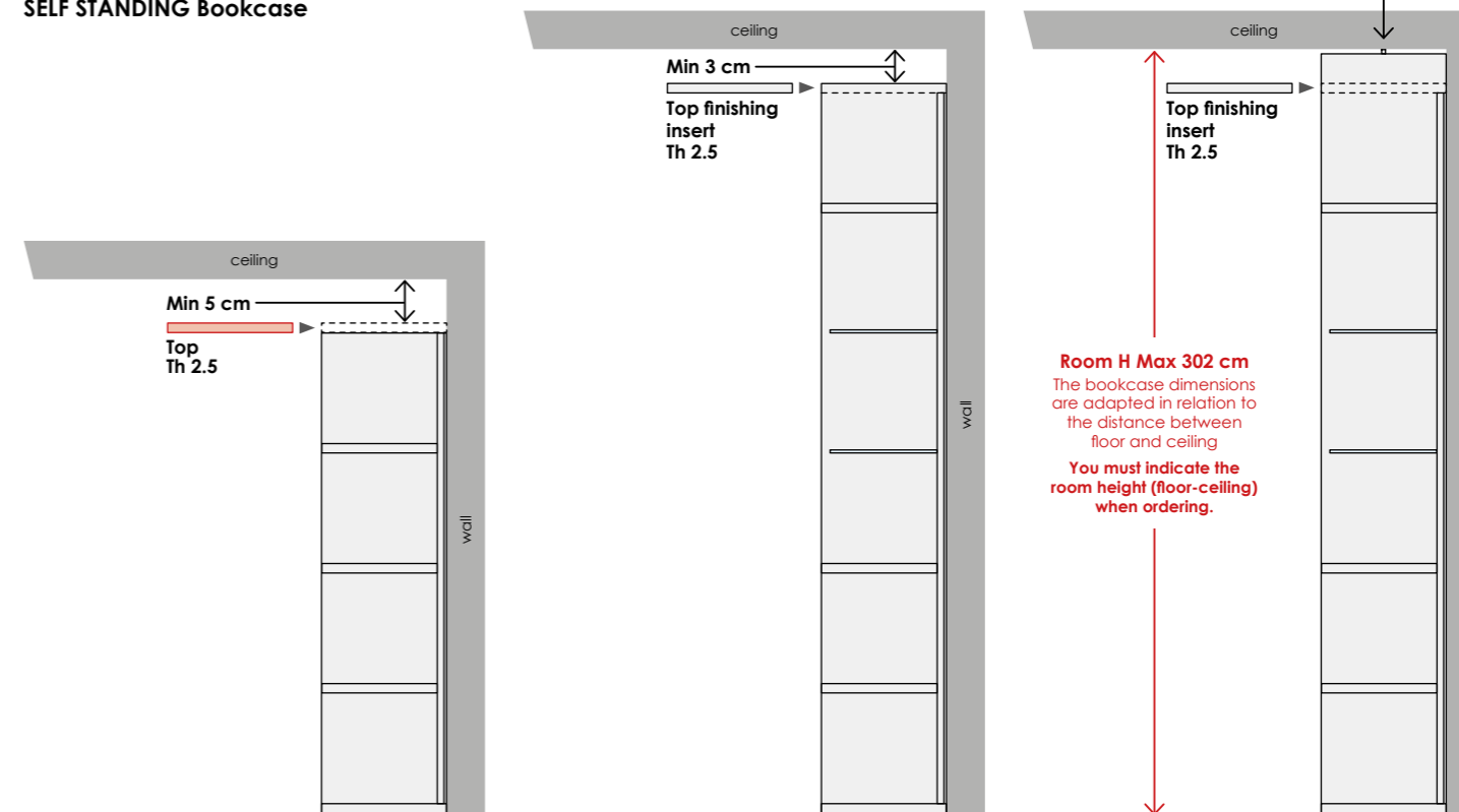
Side view with self standing Bookcase from Ht 35.3 to Ht 163.3 (included) with top finishing insert
