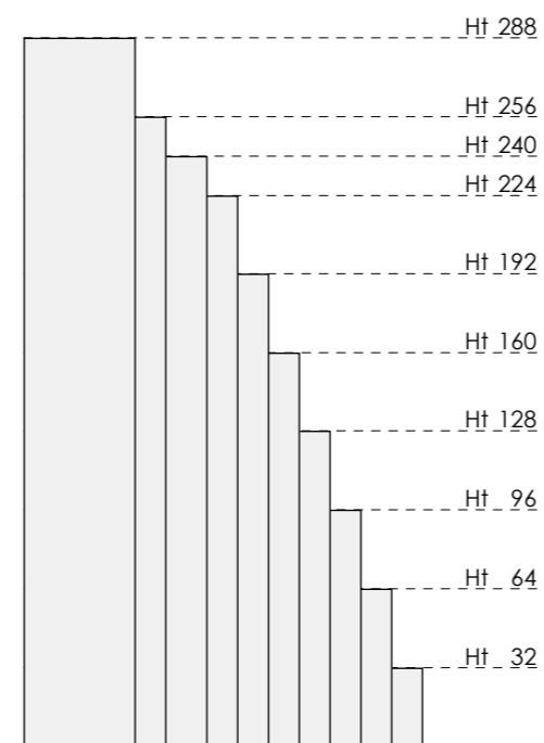
Doors W 30, 45 and 60
