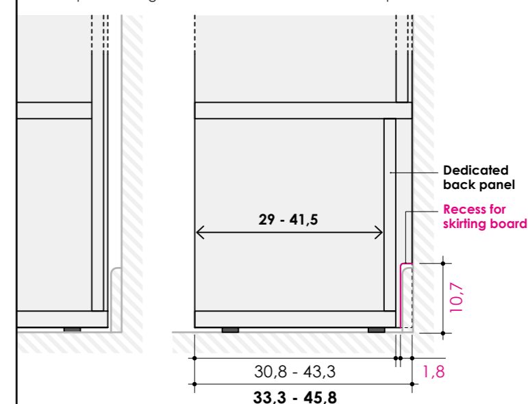
Example of skirting board recess in bookshelf with back panel:
