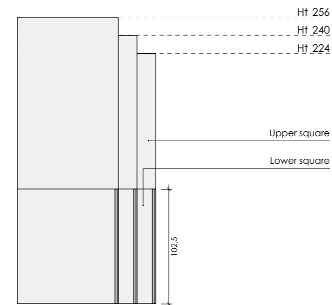
CUTTING melamine-coated doors W 90, 100 and 135
