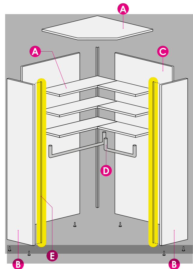
SMALL walk-in wardrobe
