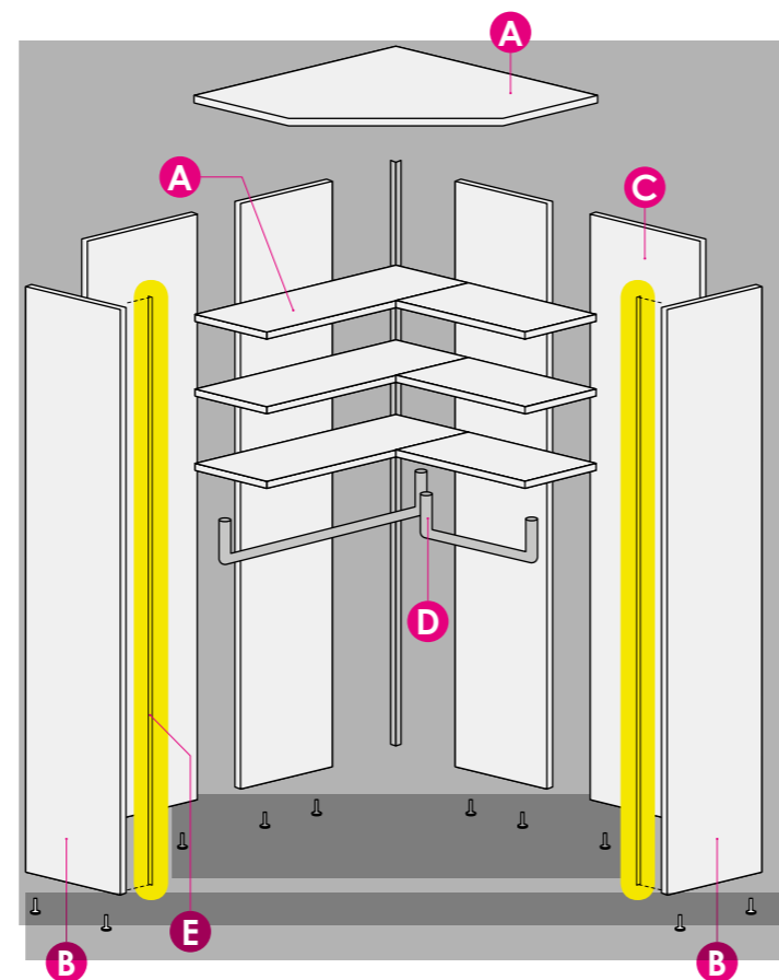
BIG walk-in wardrobe
