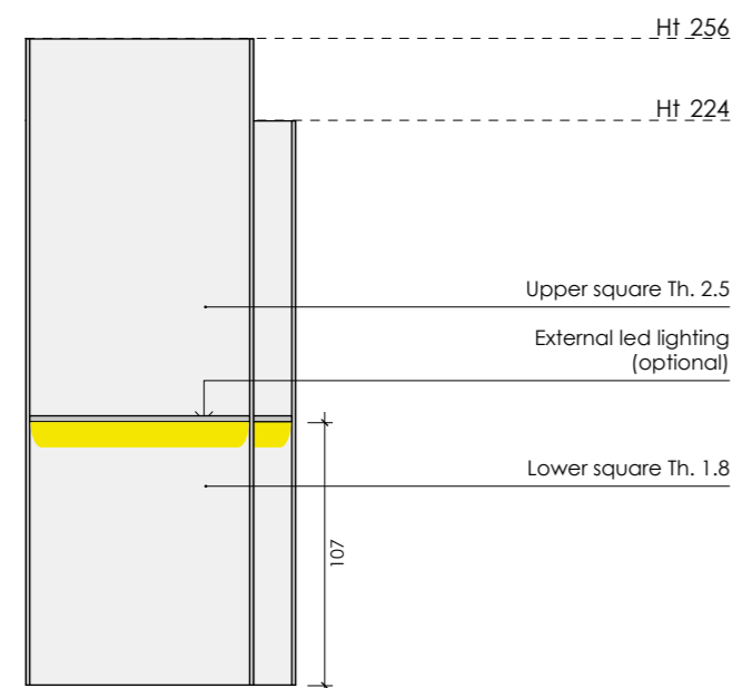
RAIL melamine-coated doors W 90, 100 and 135
