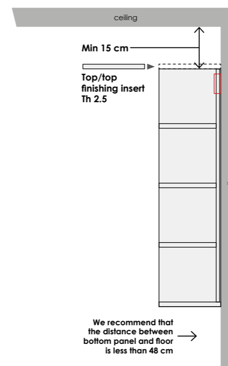
Side view with suspended Bookcase
