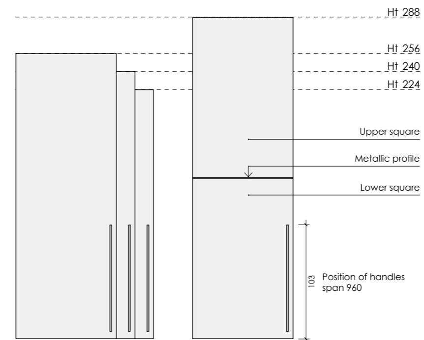
CONCRETA melamine-coated doors W 90 and 100
