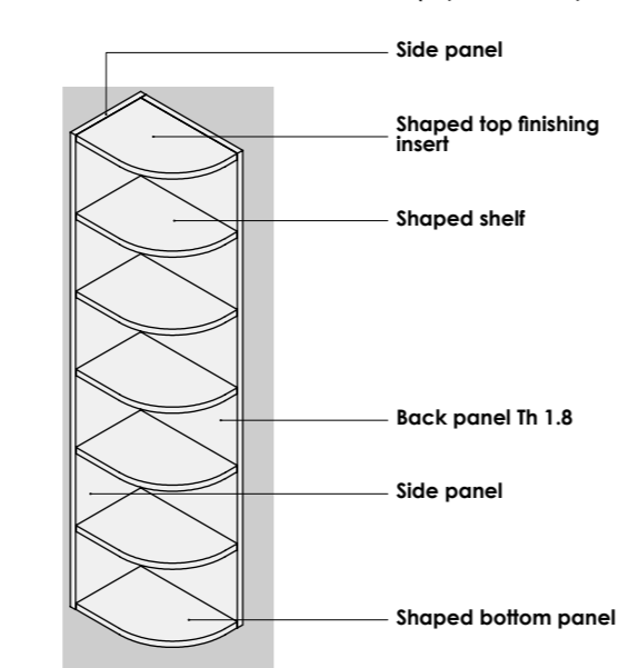
Curved bookcase end unit (Dpt 33.3/Dpt 45.8)
