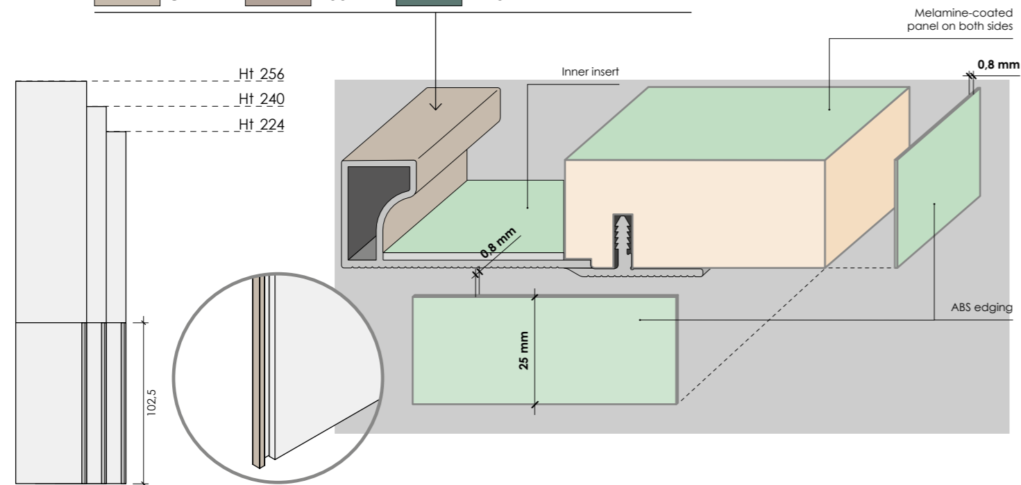
Doors W 45, 50 and 60
