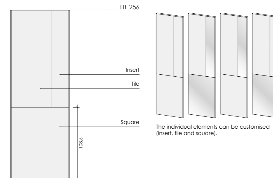
MOSAICO melamine-coated doors/Mirror doors W 90, 100 and 135
