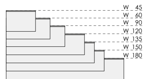
Folding doors Ht 32
