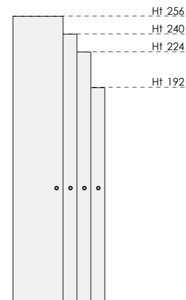
Doors with bar lock W 45 and 60
