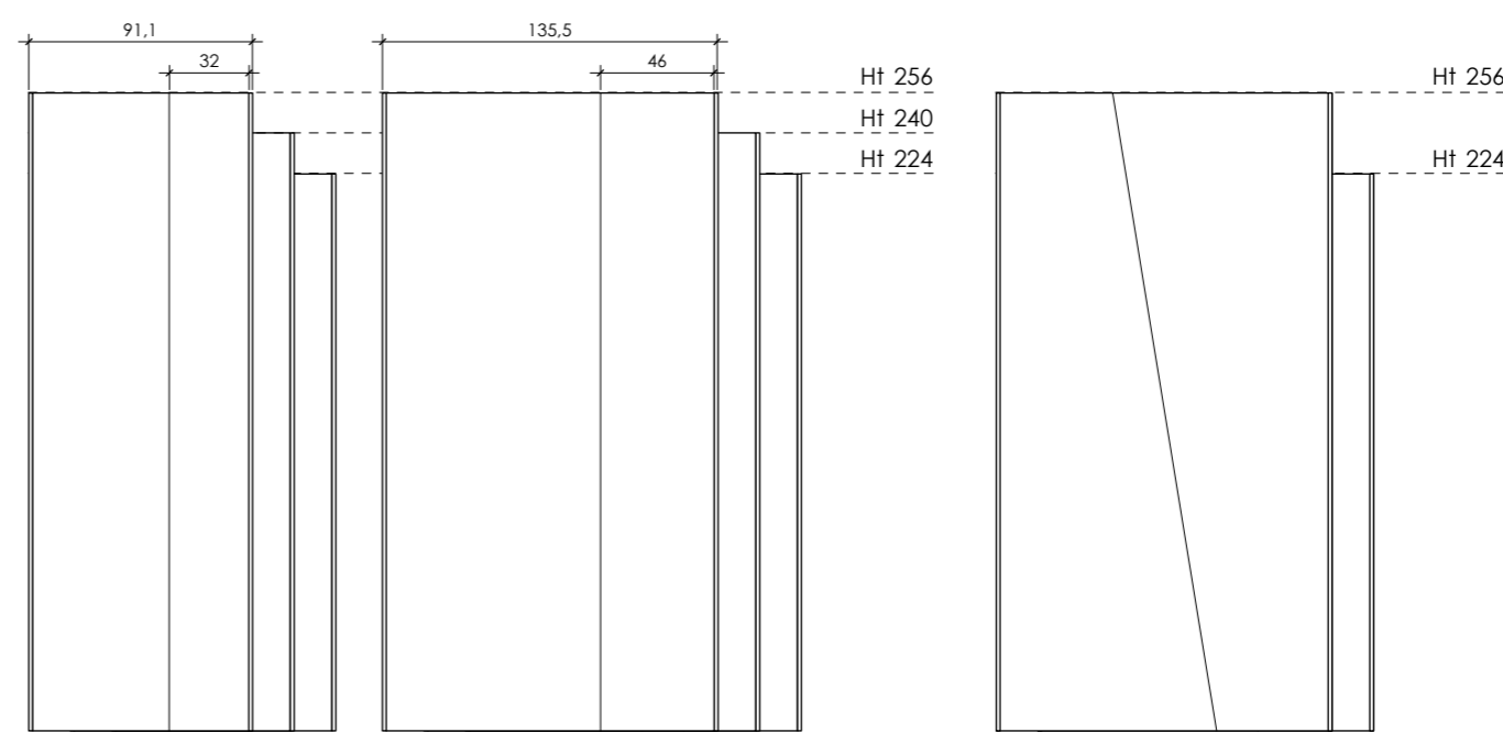
SECTOR melamine-coated doors W 91.1 and 135.5
