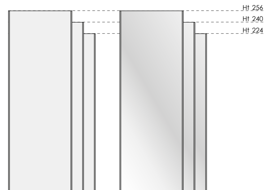
STYLE melamine-coated doors/Mirror doors W 90 and 100
