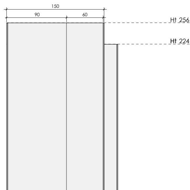
FREEDOM melamine-coated doors W 150
