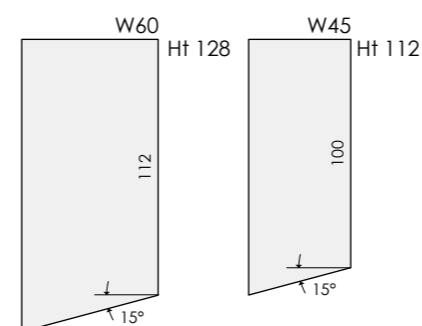
Doors with oblique cut
