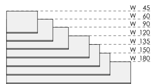
Flap doors Ht 32
