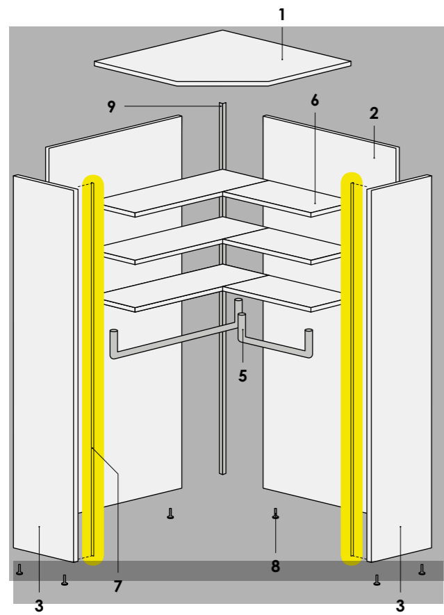
SMALL walk-in wardrobe 98.7 x 98.7
