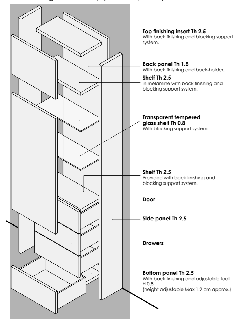
Self standing bookcase (Dpt 33.3/Dpt 45.8)
