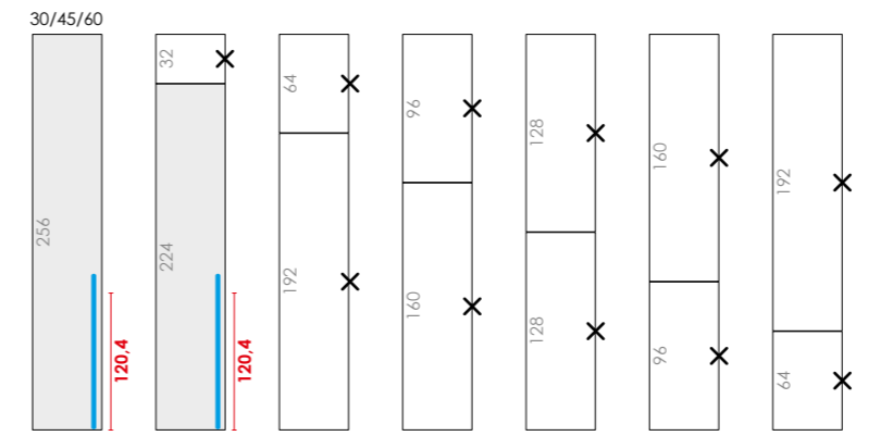
Schema maniglie TALL TALL handles diagram
