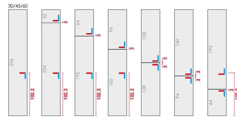
Schema maniglie BLADE BLADE handles diagram
